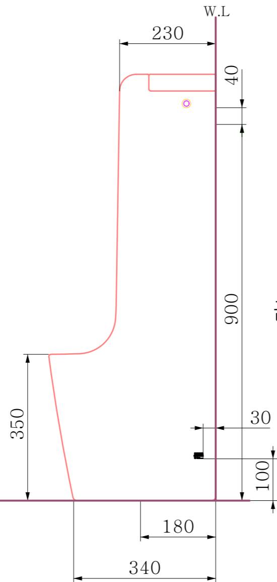
SIDE - RIGHT
